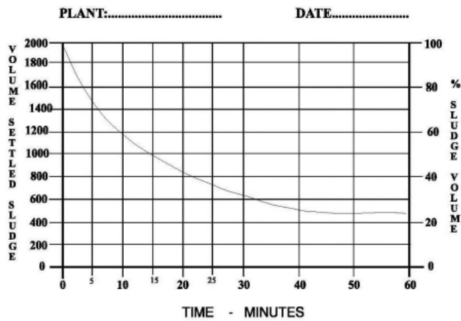
FIGURE B - SETTLEOMETER GRAPH
