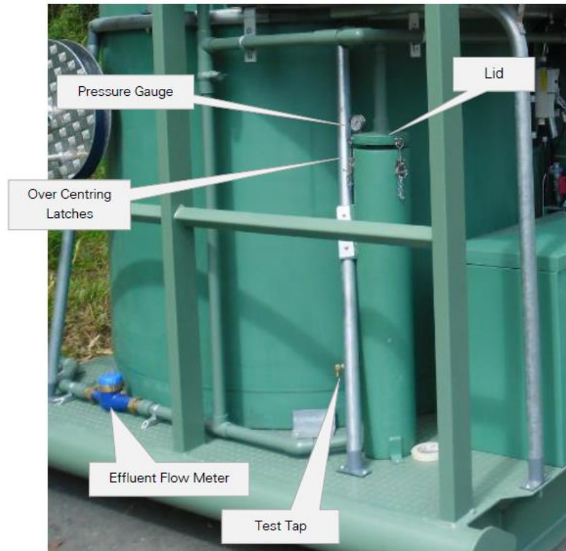
Photo 2. Sock Filter and Effluent Outlet Pipe Work
