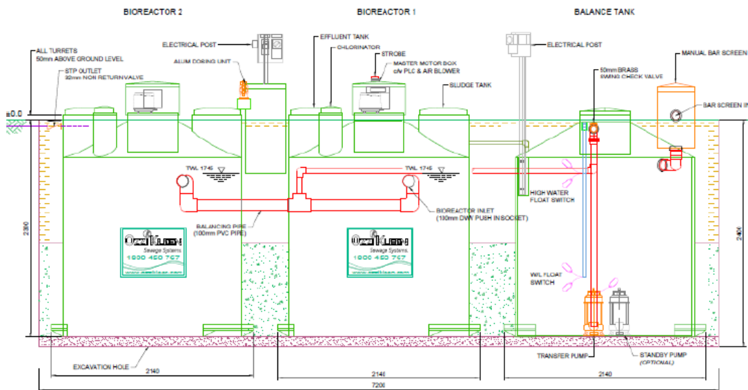
Figure 2. RP20A Below Ground Treatment Plant
