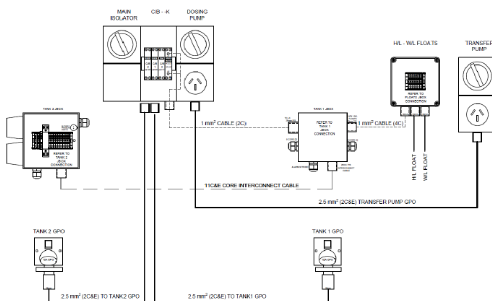
Figure 4. Electrical Connections Required at Installation
