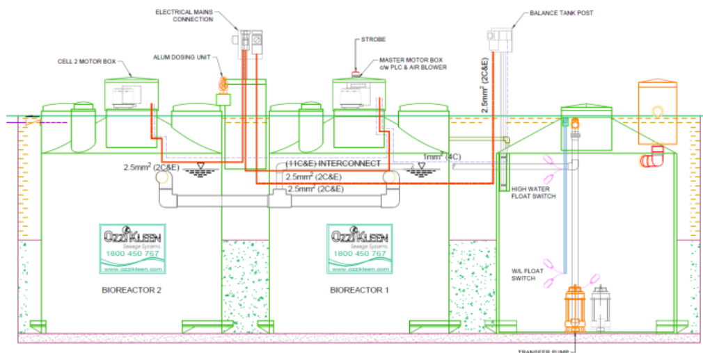
Figure 3. RP20A INTER CONNECTION ELECTRICAL LAYOUT
