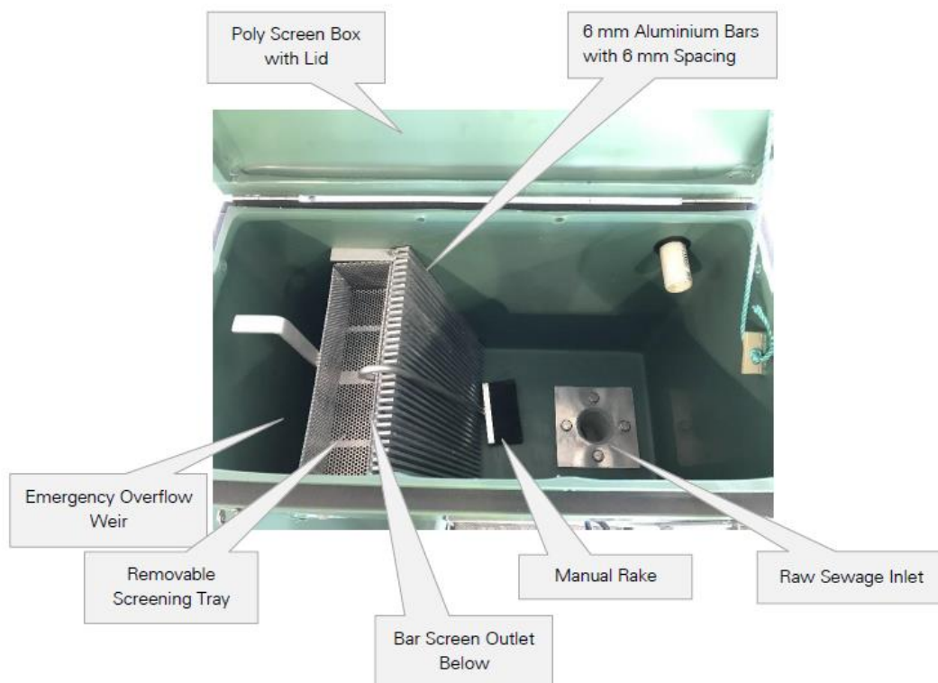
Photo 1. Manual Bar Screen Internal
